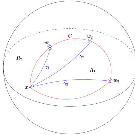
Figure 3: The loop C at a basepoint x through points of B [Cas19].
