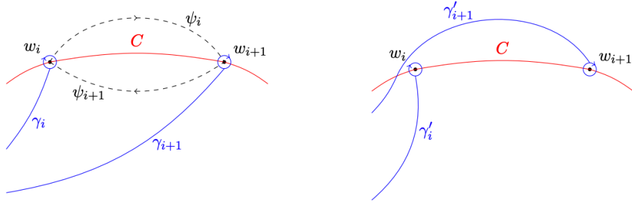
Figure 4: Computing \tilde{\psi}(1) by deforming \gamma_i along \psi_i [Cas19].
