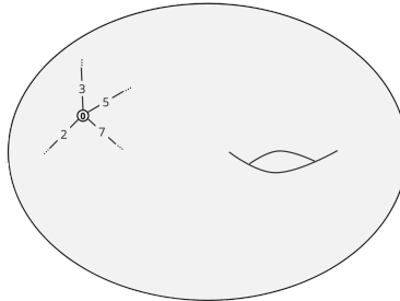
Figure 1: Diagram shows \sigma_0 has cycle (3\ 2\ 7\ 5) induced by the orientation on X .
